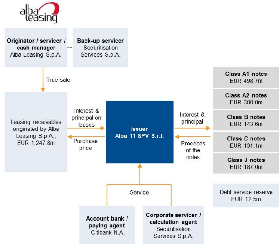
Figure 1: Transaction diagram
